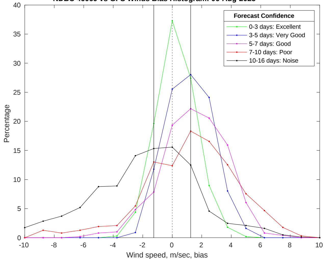
NDBC 46069 vs GFS Winds Bias Histogram: 06-Aug-2025
