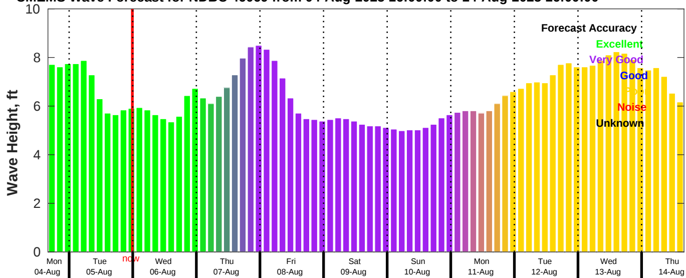
CMEMS Wave Forecast for NDBC 46069 from 04-Aug-2025 16:00:00 to 14-Aug-2025 16:00:00
