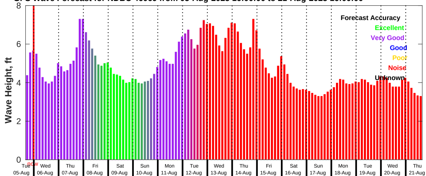
GFS Wave Forecast for NDBC 46069 from 05-Aug-2025 16:00:00 to 21-Aug-2025 16:00:00
