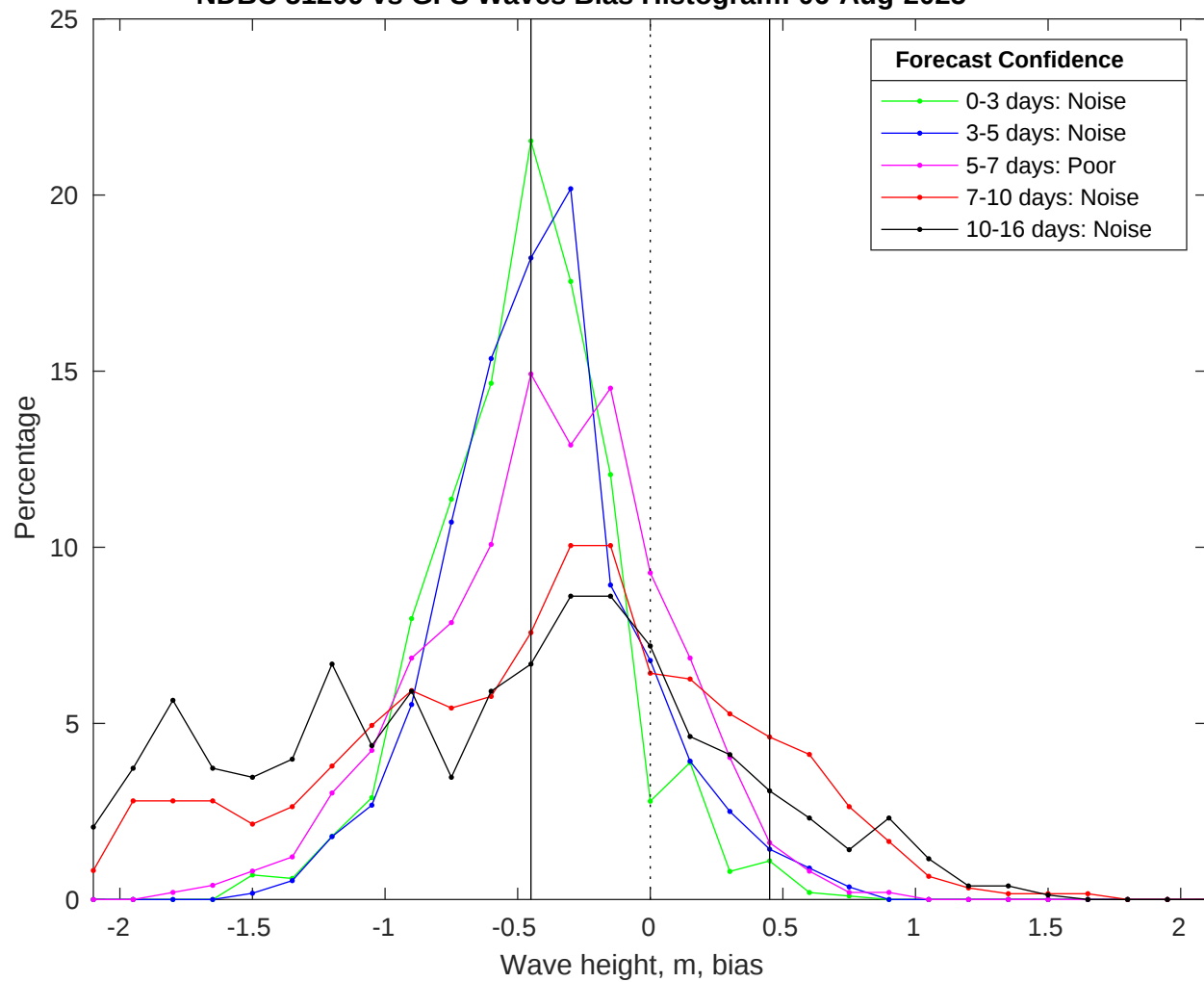
NDBC 51209 vs GFS Waves Bias Histogram: 06-Aug-2025
