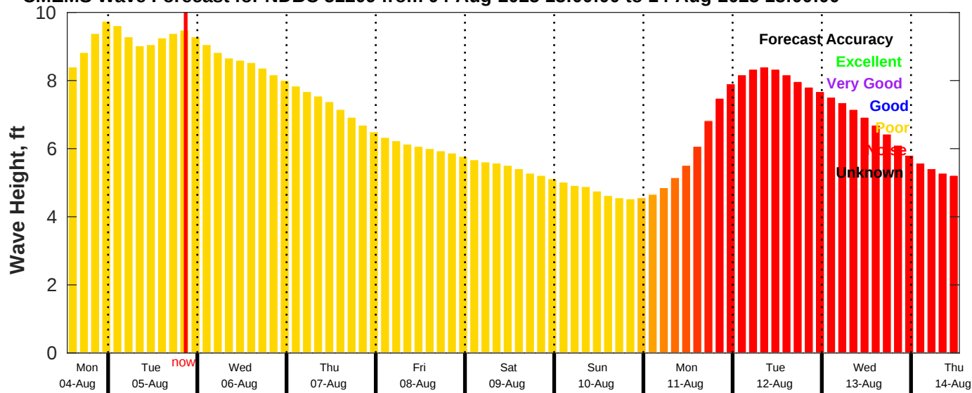
CMEMS Wave Forecast for NDBC 51209 from 04-Aug-2025 13:00:00 to 14-Aug-2025 13:00:00
