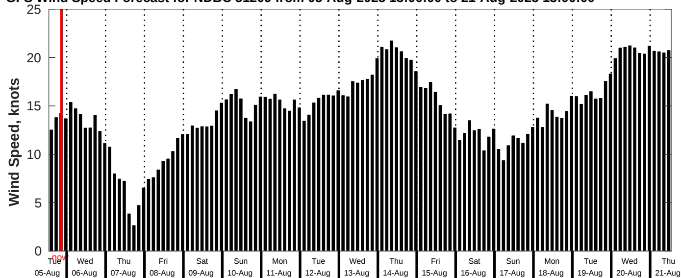
GFS Wind Speed Forecast for NDBC 51209 from 05-Aug-2025 13:00:00 to 21-Aug-2025 13:00:00
