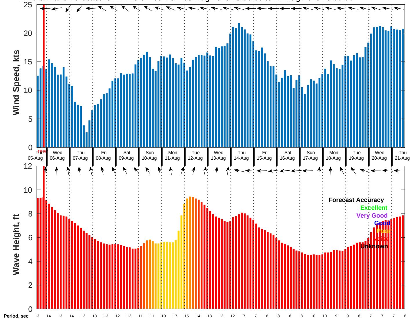
Wind & Wave Forecast for NDBC 51209 from 05-Aug-2025 13:00:00 to 21-Aug-2025 13:00:00
