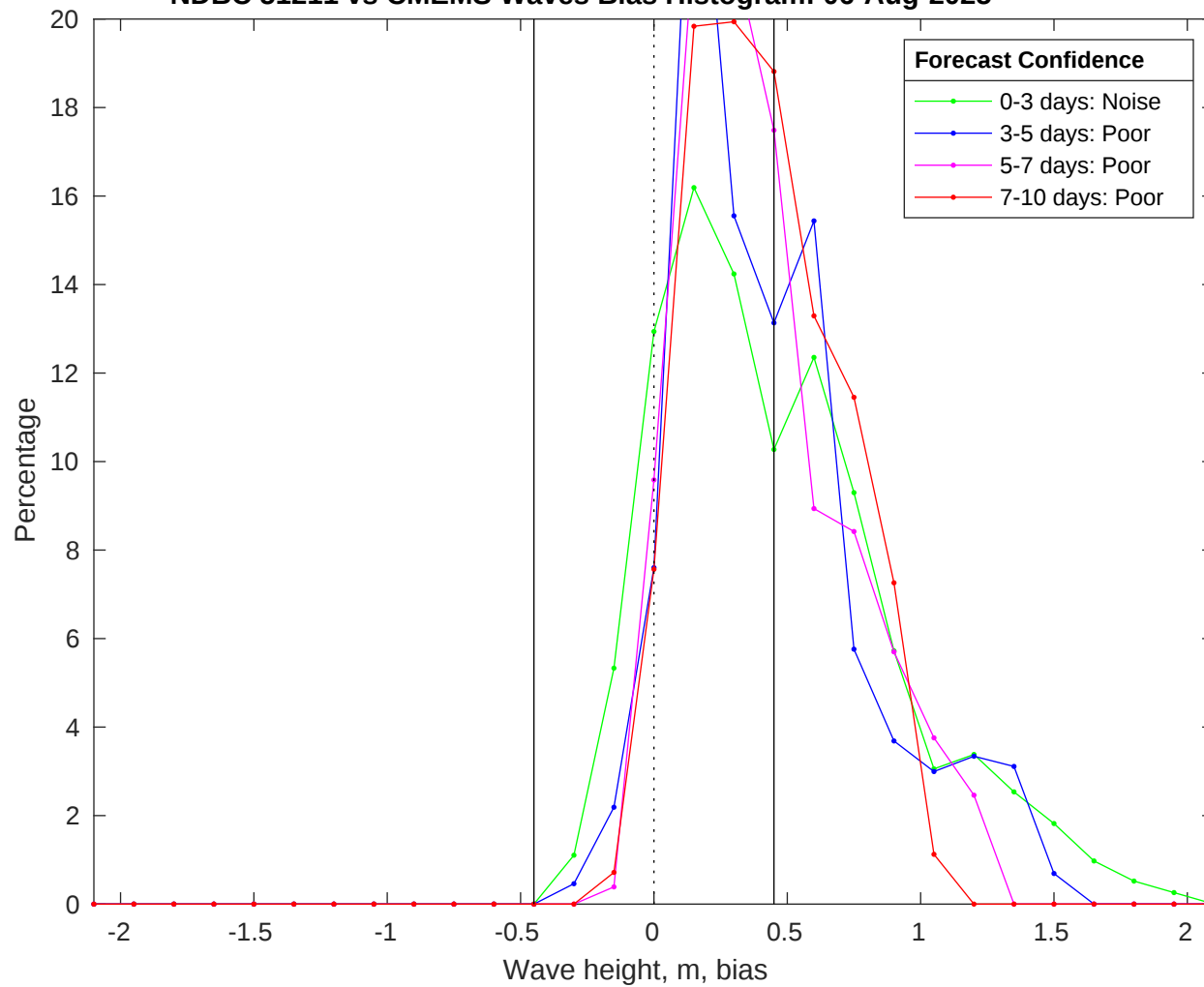
NDBC 51211 vs CMEMS Waves Bias Histogram: 06-Aug-2025
