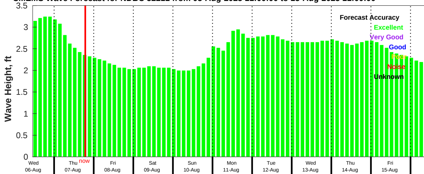
CMEMS Wave Forecast for NDBC 52211 from 05-Aug-2025 11:00:00 to 15-Aug-2025 11:00:00
