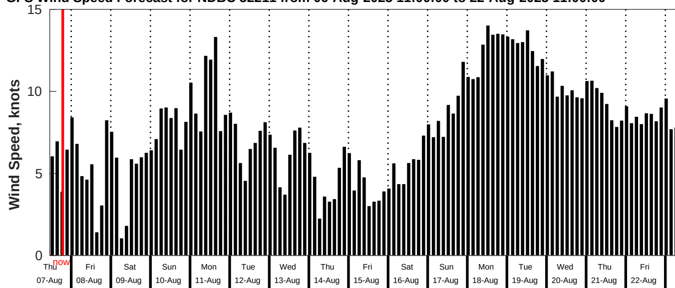
GFS Wind Speed Forecast for NDBC 52211 from 06-Aug-2025 11:00:00 to 22-Aug-2025 11:00:00
