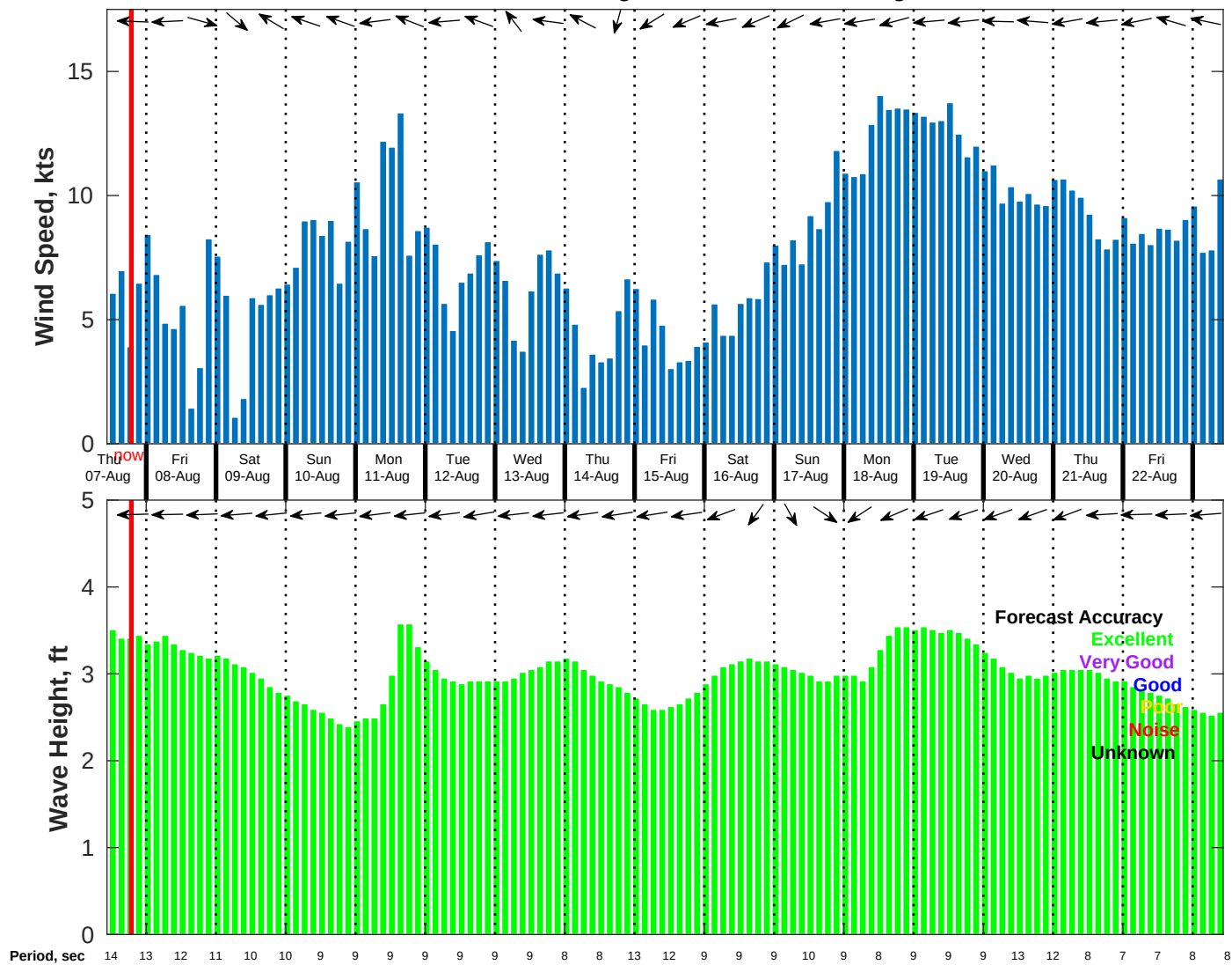
Wind & Wave Forecast for NDBC 52211 from 06-Aug-2025 11:00:00 to 22-Aug-2025 11:00:00
