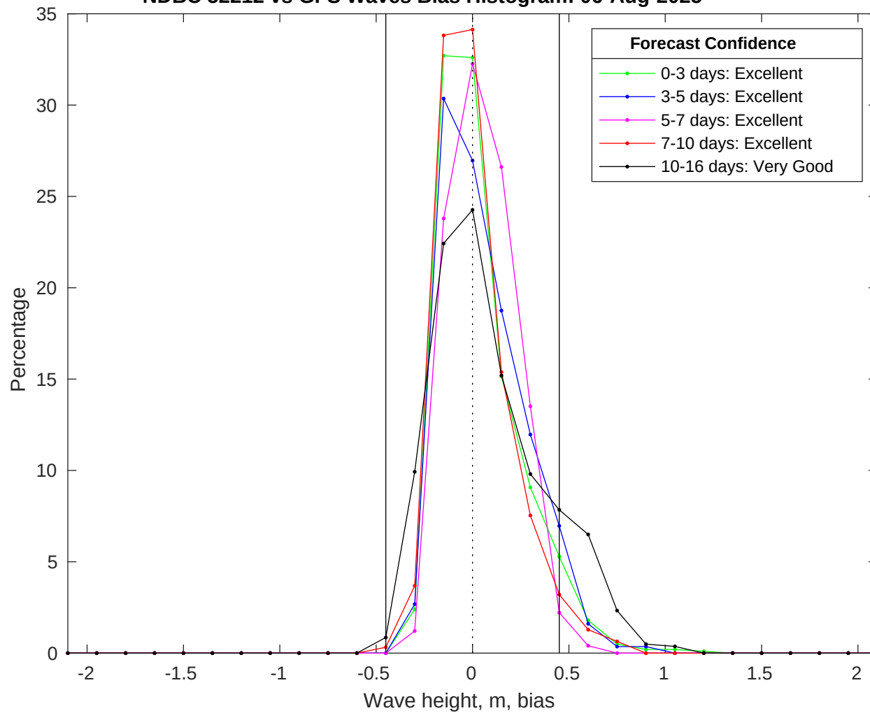
NDBC 52212 vs GFS Waves Bias Histogram: 06-Aug-2025
