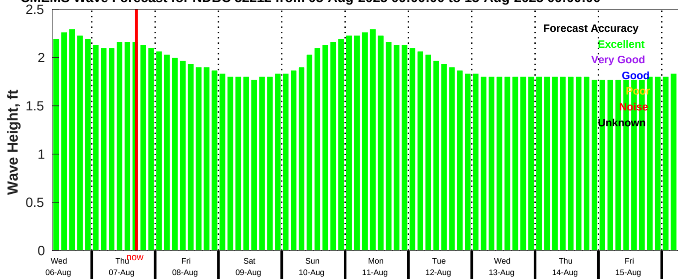
CMEMS Wave Forecast for NDBC 52212 from 05-Aug-2025 09:00:00 to 15-Aug-2025 09:00:00
