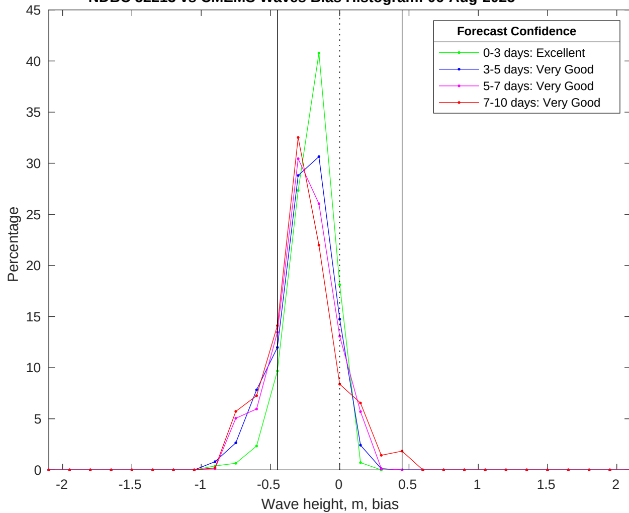
NDBC 52213 vs CMEMS Waves Bias Histogram: 06-Aug-2025
