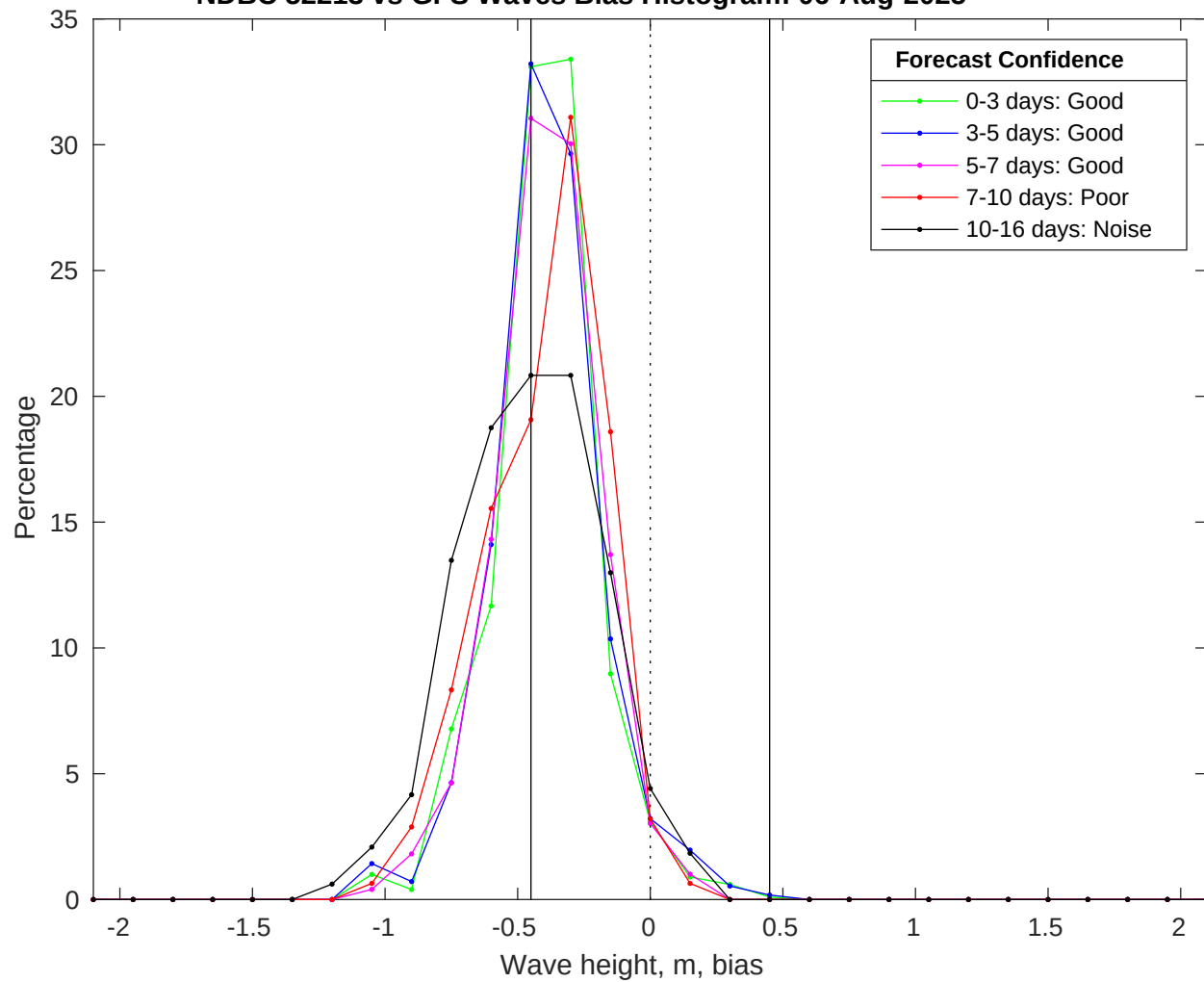
NDBC 52213 vs GFS Waves Bias Histogram: 06-Aug-2025
