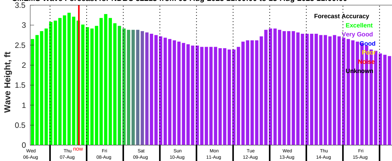
CMEMS Wave Forecast for NDBC 52213 from 05-Aug-2025 11:00:00 to 15-Aug-2025 11:00:00
