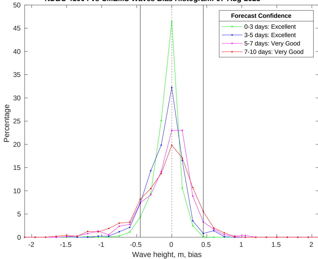
NDBC 41004 vs CMEMS Waves Bias Histogram: 07-Aug-2025
