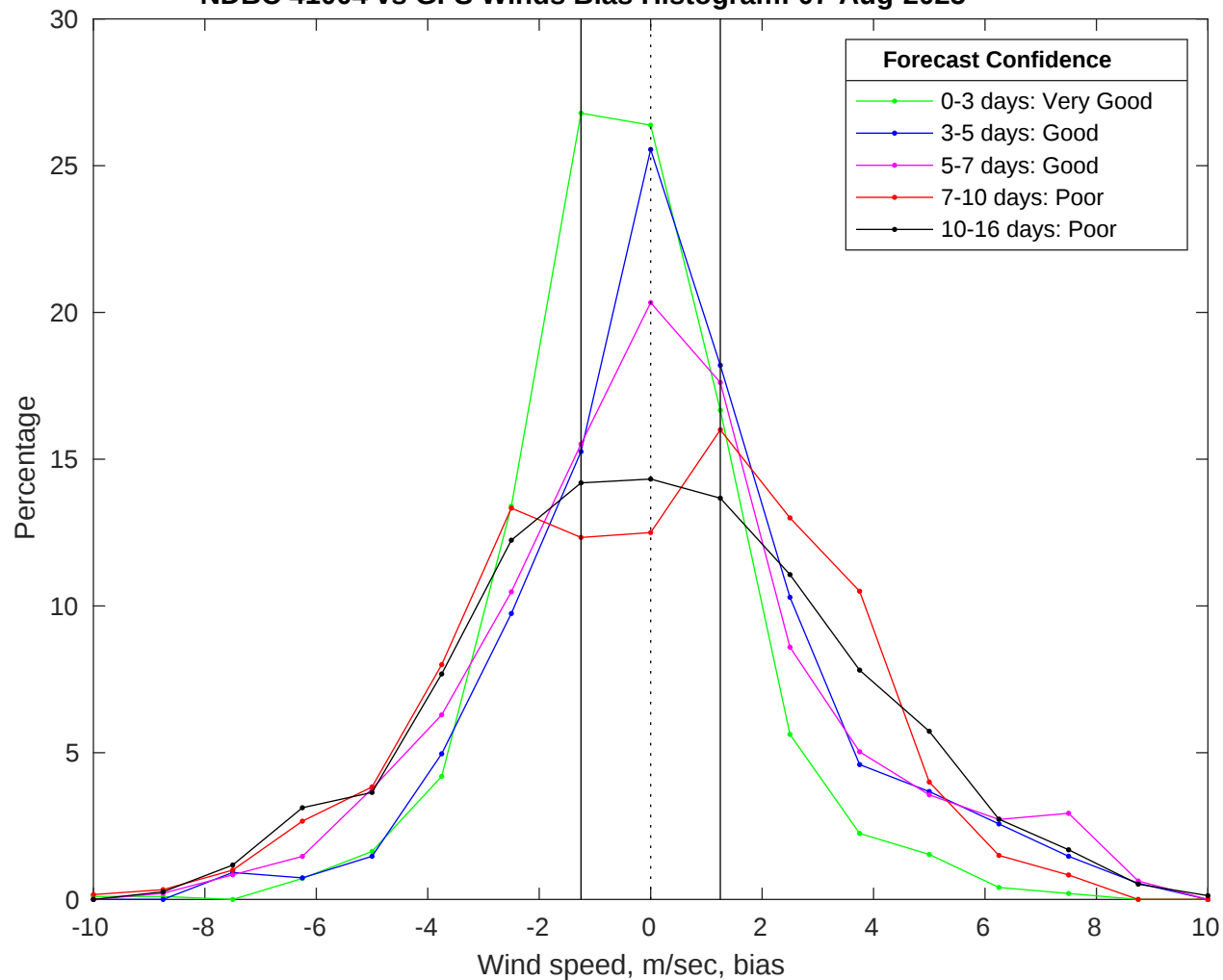
NDBC 41004 vs GFS Winds Bias Histogram: 07-Aug-2025
