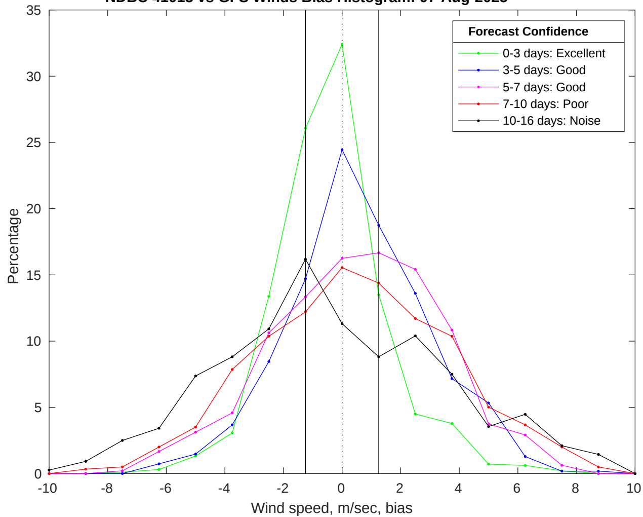
NDBC 41013 vs GFS Winds Bias Histogram: 07-Aug-2025
