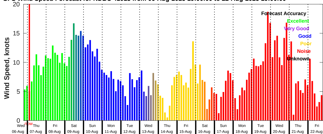
GFS Wind Speed Forecast for NDBC 41013 from 06-Aug-2025 19:00:00 to 22-Aug-2025 19:00:00
