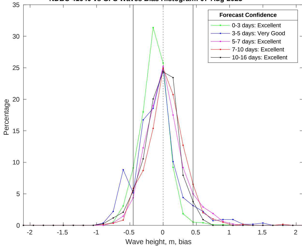
NDBC 41040 vs GFS Waves Bias Histogram: 07-Aug-2025
