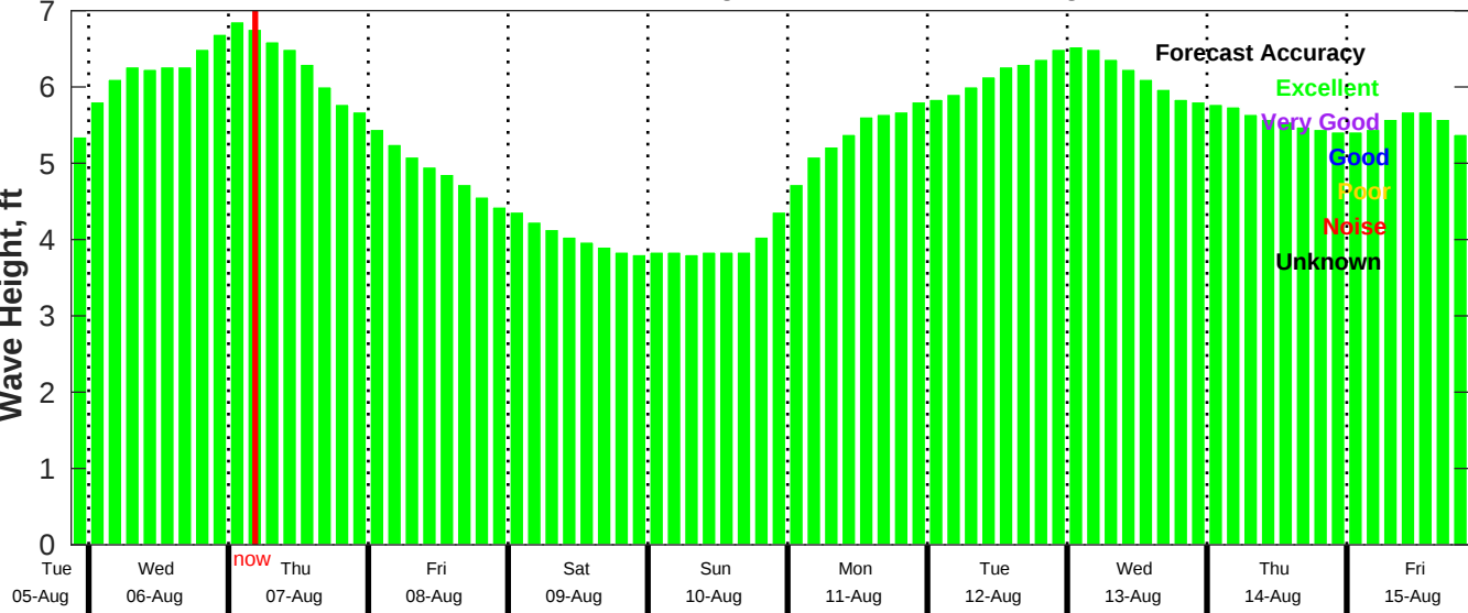
CMEMS Wave Forecast for NDBC 41040 from 05-Aug-2025 21:00:00 to 15-Aug-2025 21:00:00
