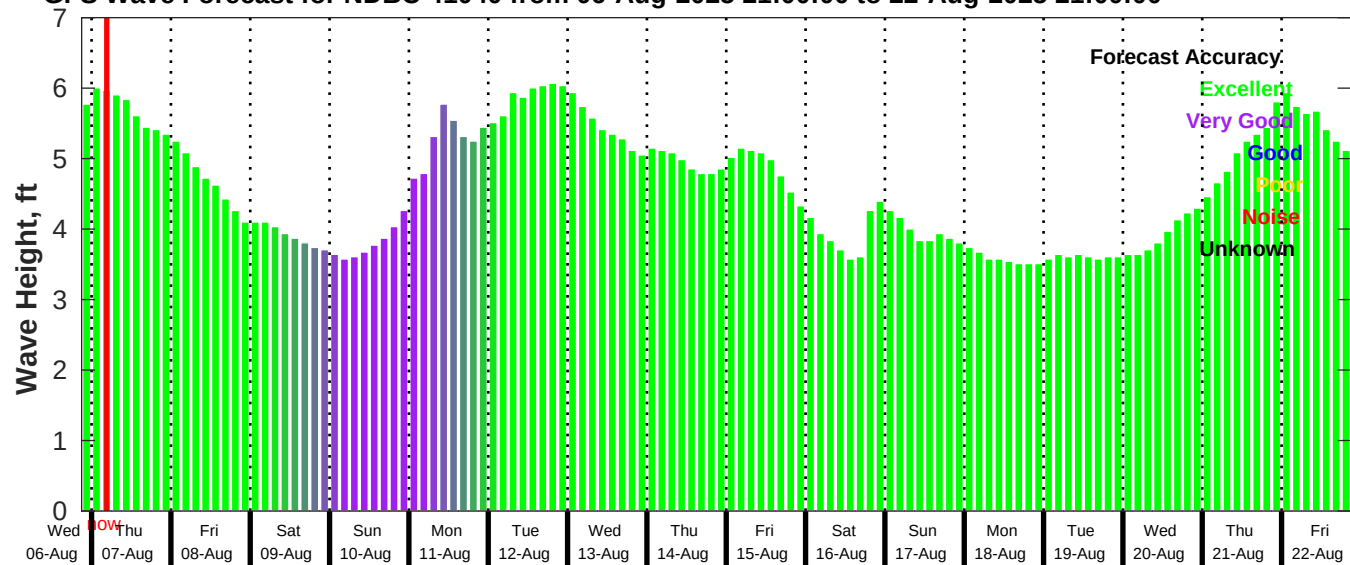
GFS Wave Forecast for NDBC 41040 from 06-Aug-2025 21:00:00 to 22-Aug-2025 21:00:00
