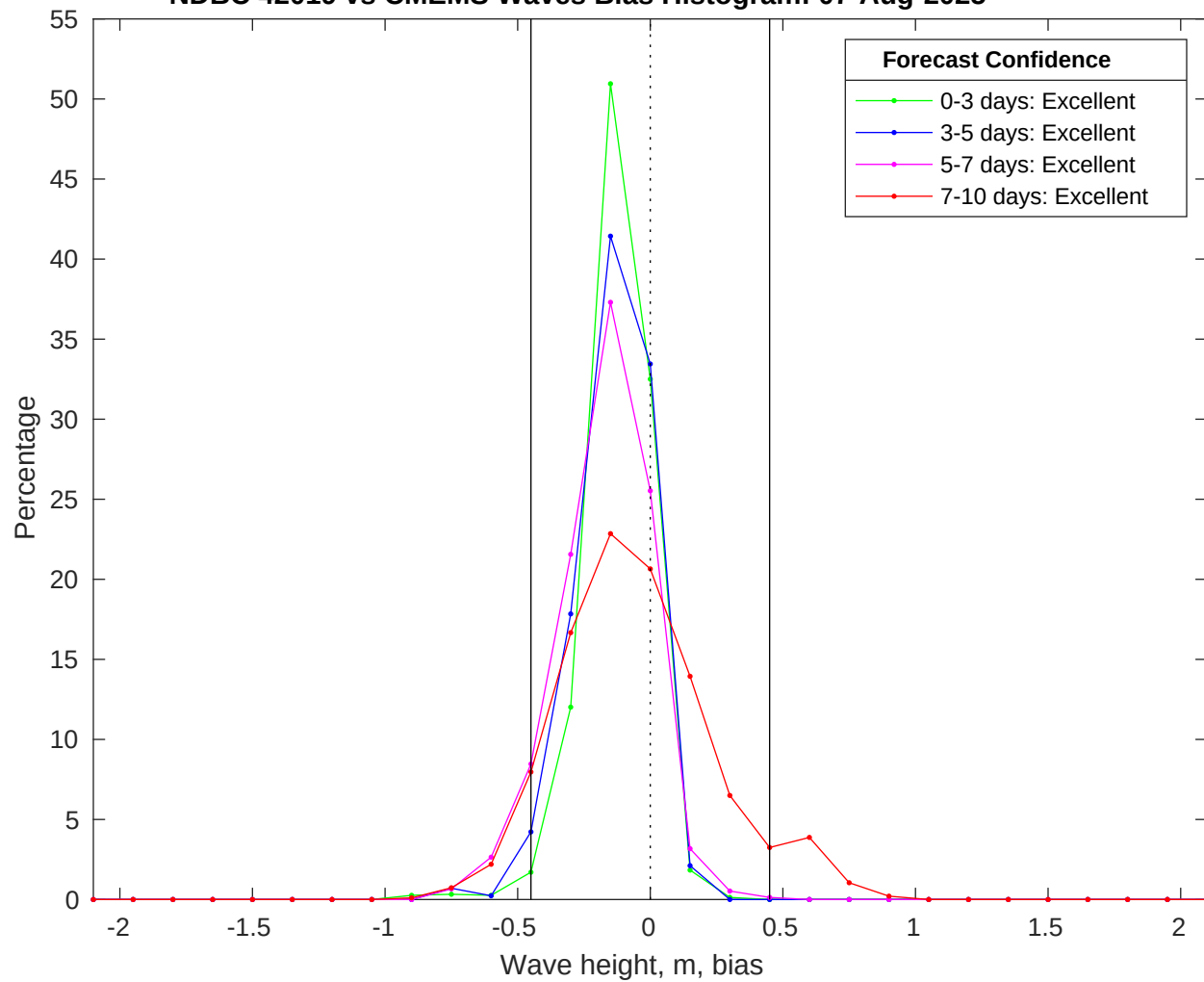
NDBC 42019 vs CMEMS Waves Bias Histogram: 07-Aug-2025
