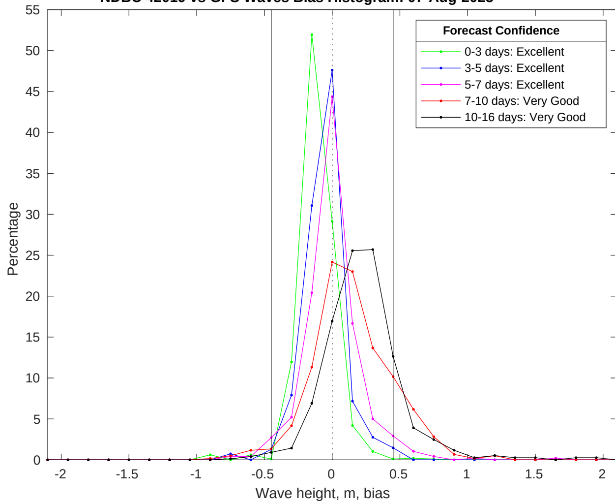
NDBC 42019 vs GFS Waves Bias Histogram: 07-Aug-2025
