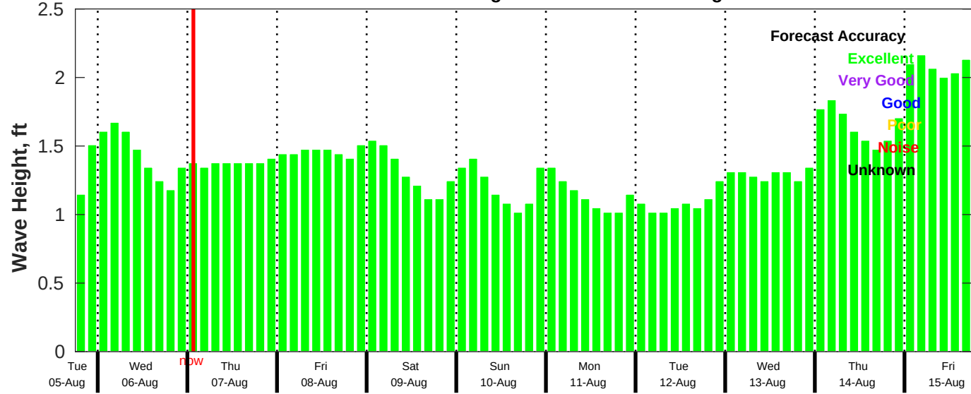
CMEMS Wave Forecast for NDBC 42019 from 05-Aug-2025 18:00:00 to 15-Aug-2025 18:00:00
