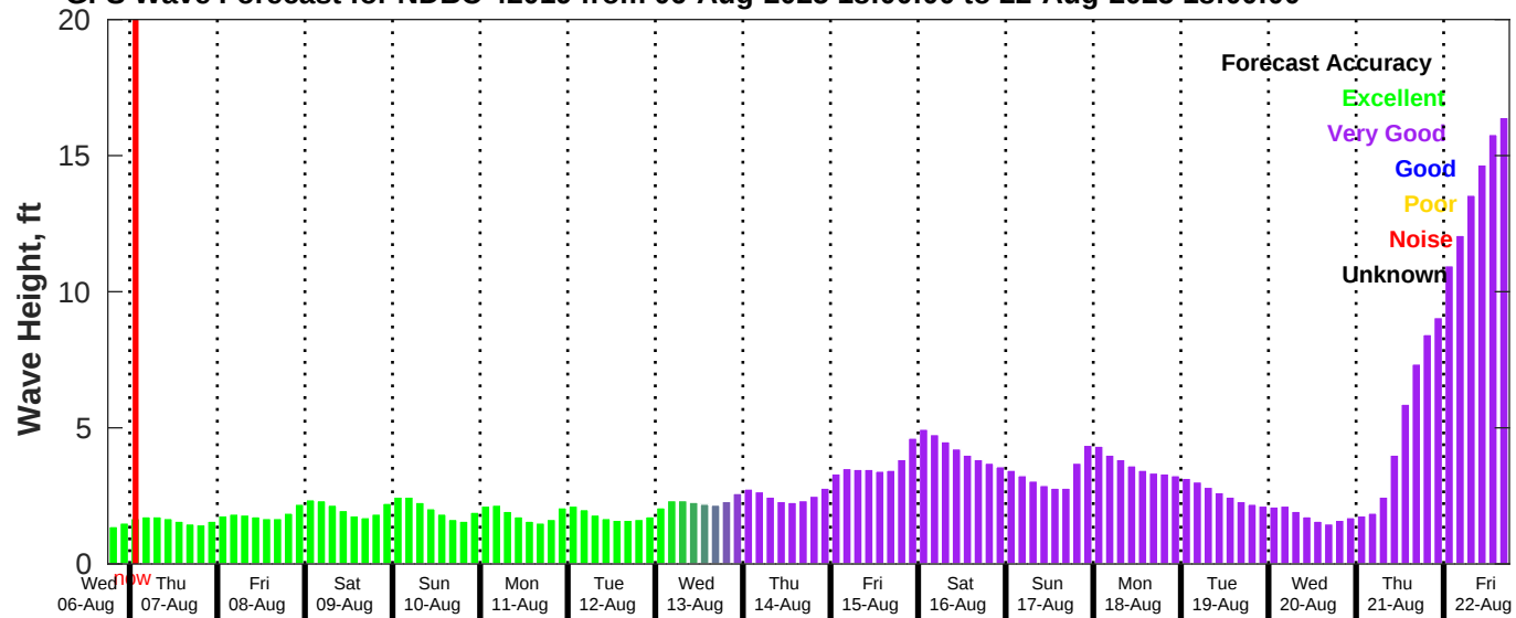
GFS Wave Forecast for NDBC 42019 from 06-Aug-2025 18:00:00 to 22-Aug-2025 18:00:00
