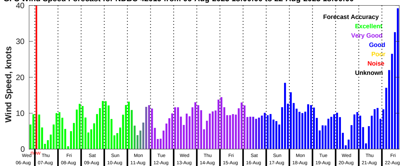
GFS Wind Speed Forecast for NDBC 42019 from 06-Aug-2025 18:00:00 to 22-Aug-2025 18:00:00
