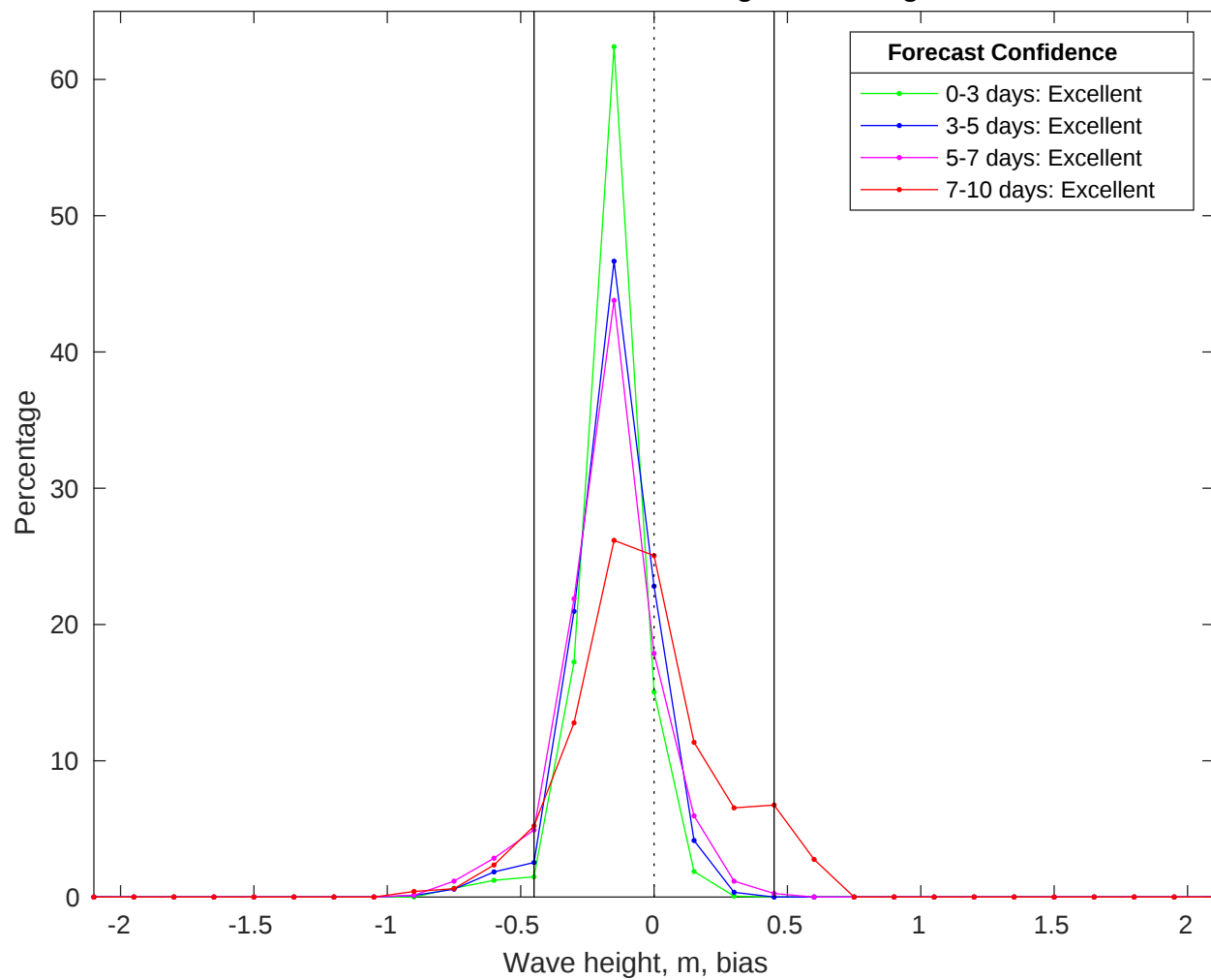
NDBC 42035 vs CMEMS Waves Bias Histogram: 07-Aug-2025
