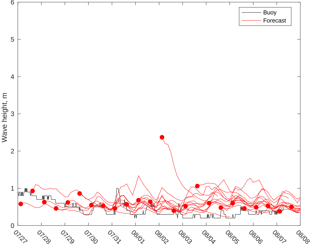
NDBC 42035 vs GFS Waves: 10 to 16 day forecast
