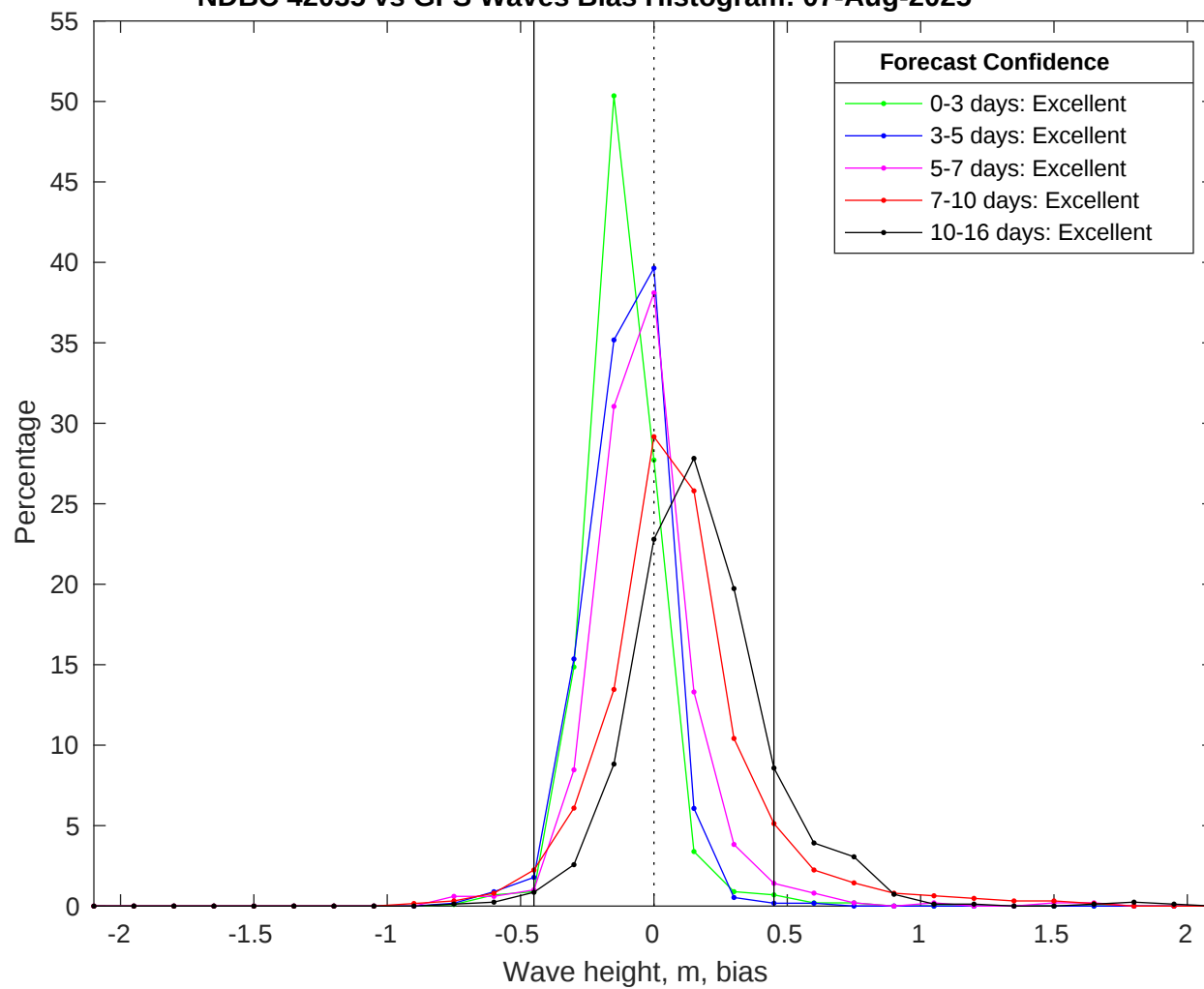
NDBC 42035 vs GFS Waves Bias Histogram: 07-Aug-2025
