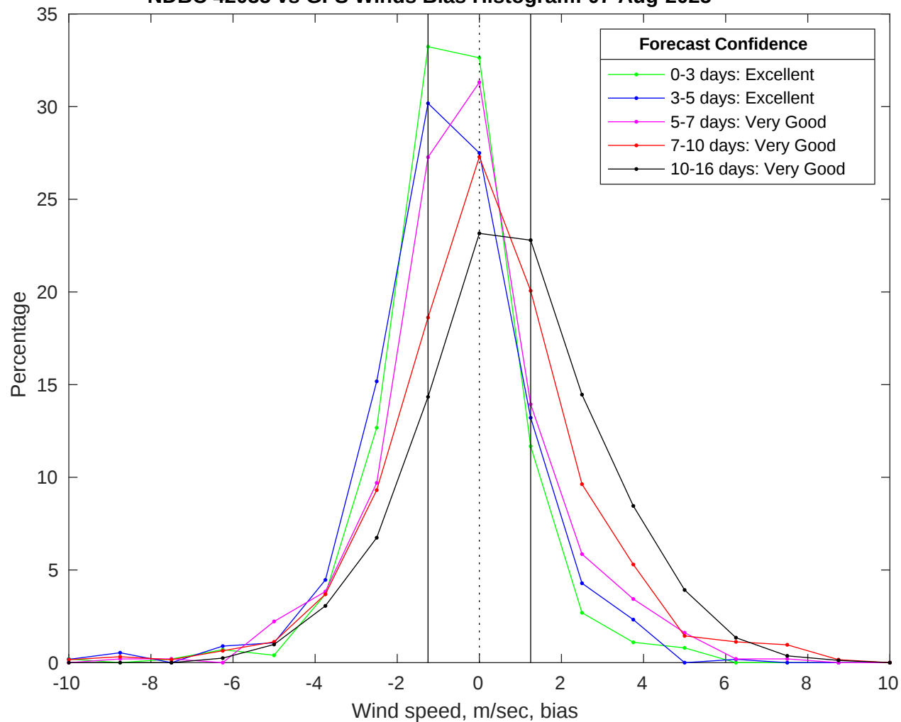
NDBC 42035 vs GFS Winds Bias Histogram: 07-Aug-2025
