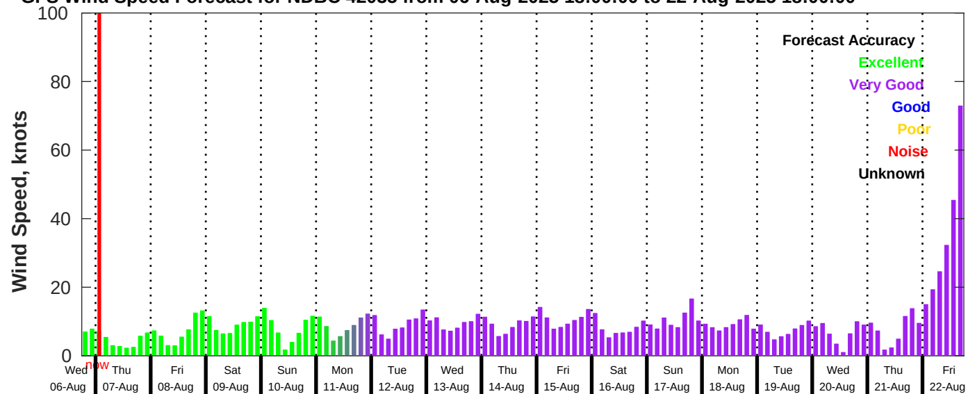
GFS Wind Speed Forecast for NDBC 42035 from 06-Aug-2025 18:00:00 to 22-Aug-2025 18:00:00
