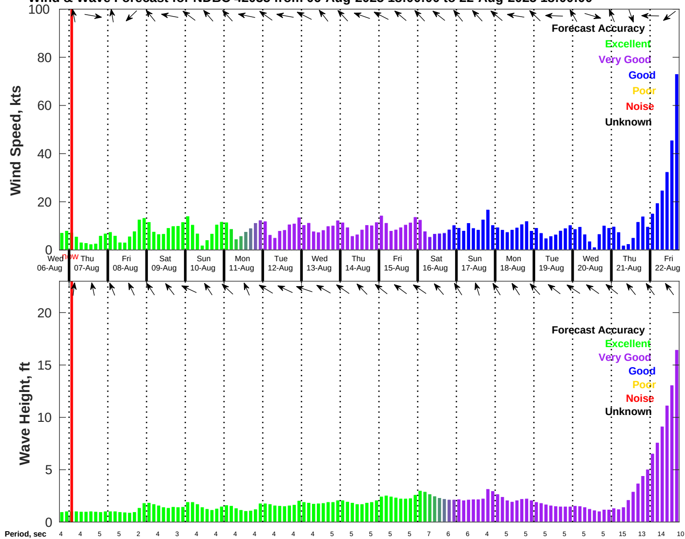
Wind & Wave Forecast for NDBC 42035 from 06-Aug-2025 18:00:00 to 22-Aug-2025 18:00:00
