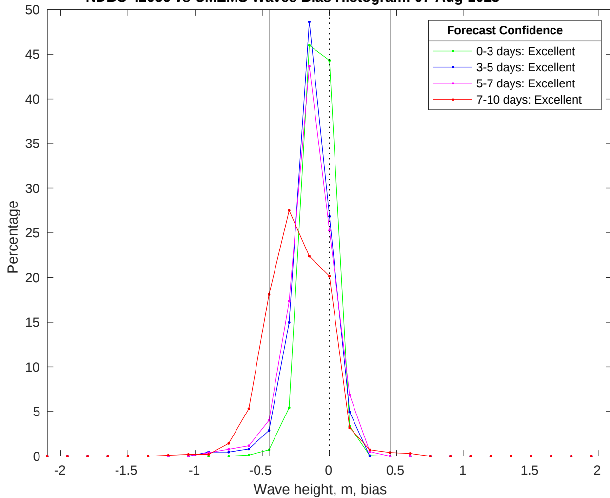
NDBC 42036 vs CMEMS Waves Bias Histogram: 07-Aug-2025
