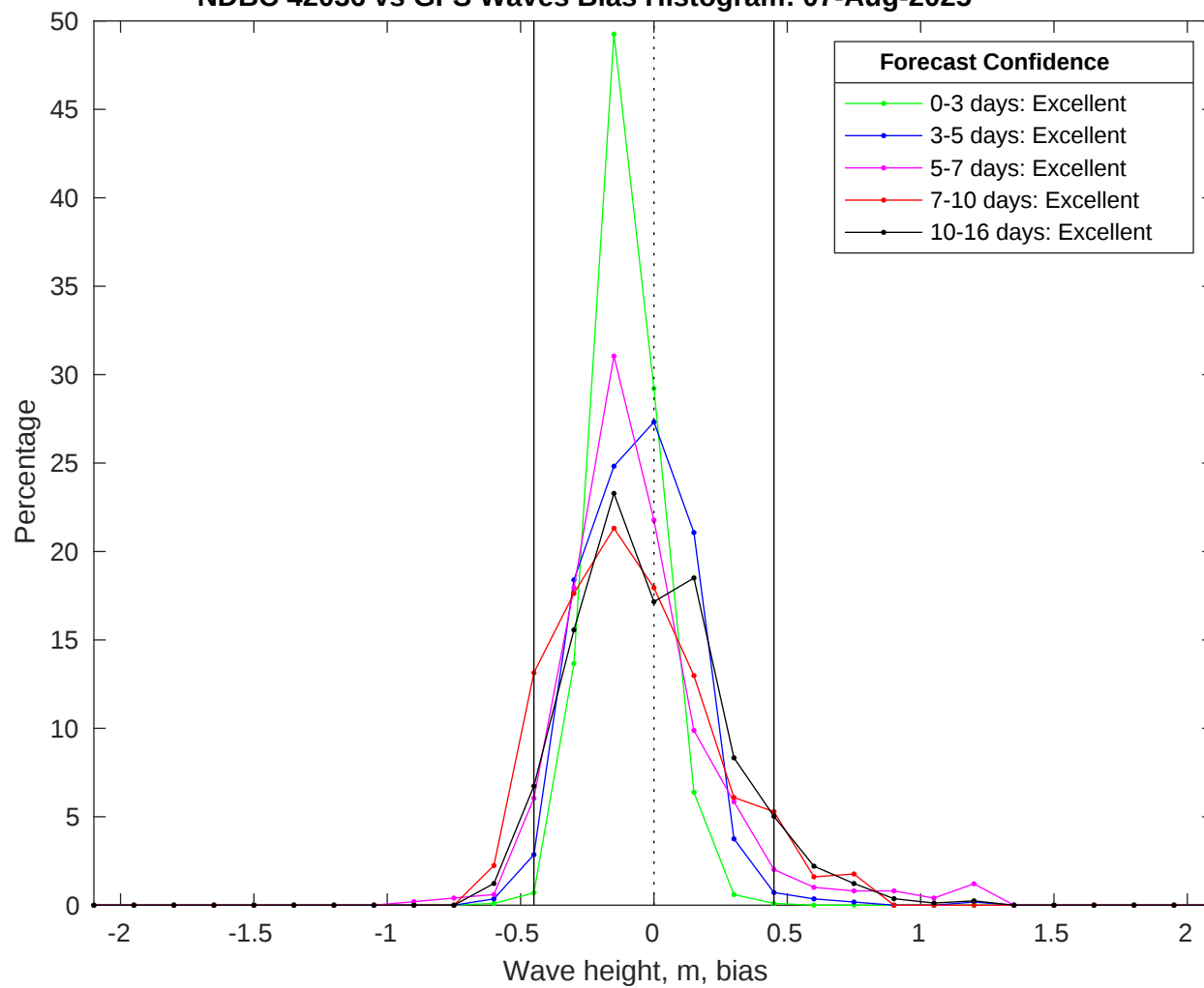
NDBC 42036 vs GFS Waves Bias Histogram: 07-Aug-2025
