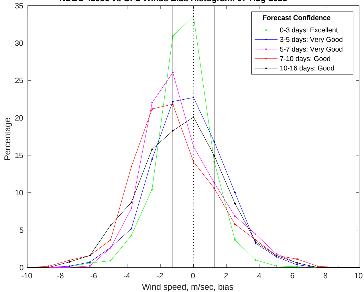
NDBC 42036 vs GFS Winds Bias Histogram: 07-Aug-2025
