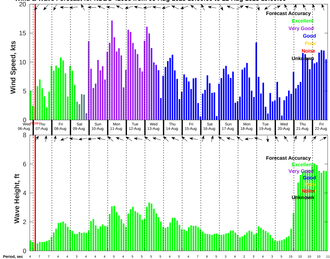
Wind & Wave Forecast for NDBC 42036 from 06-Aug-2025 19:00:00 to 22-Aug-2025 19:00:00
