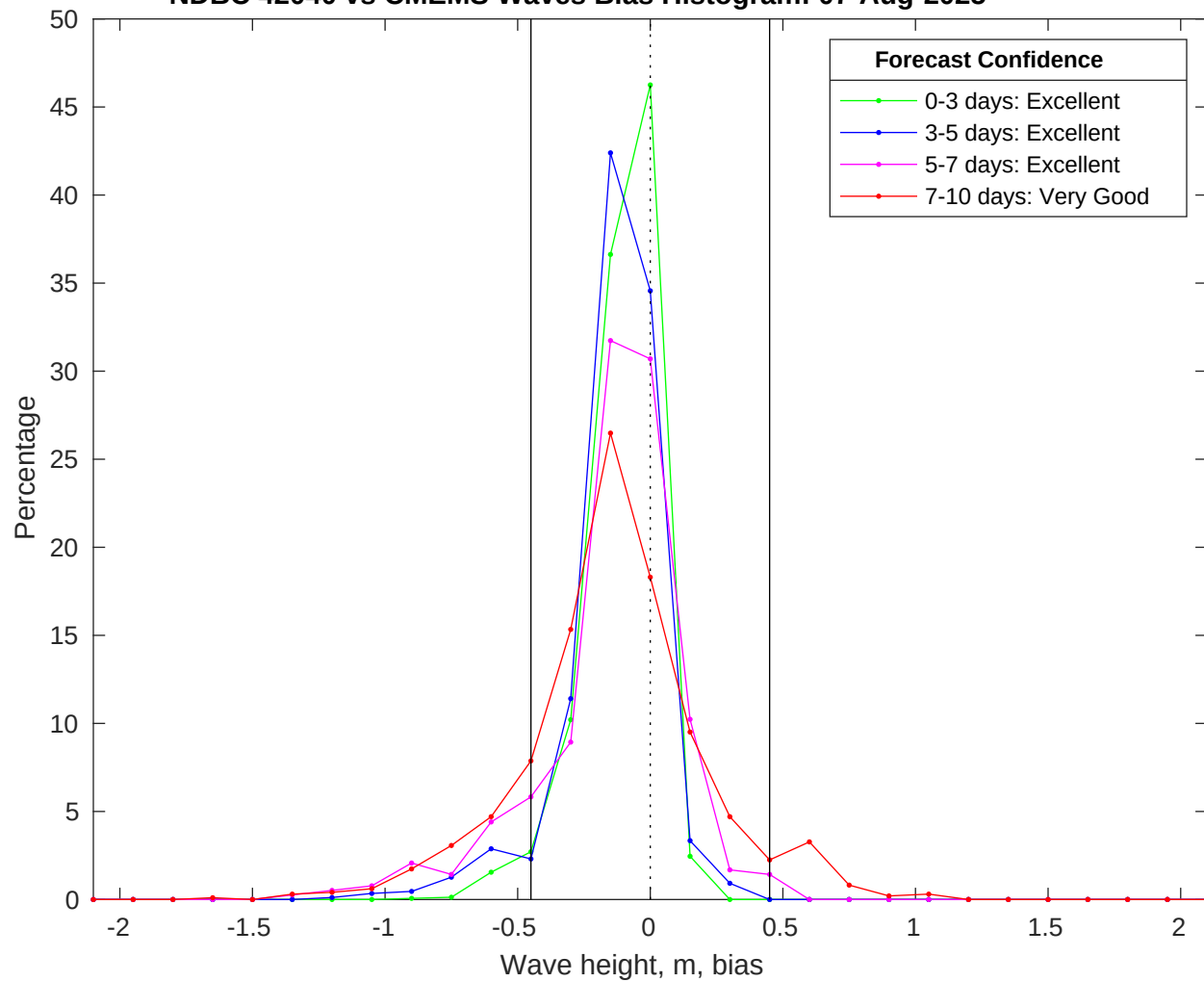
NDBC 42040 vs CMEMS Waves Bias Histogram: 07-Aug-2025
