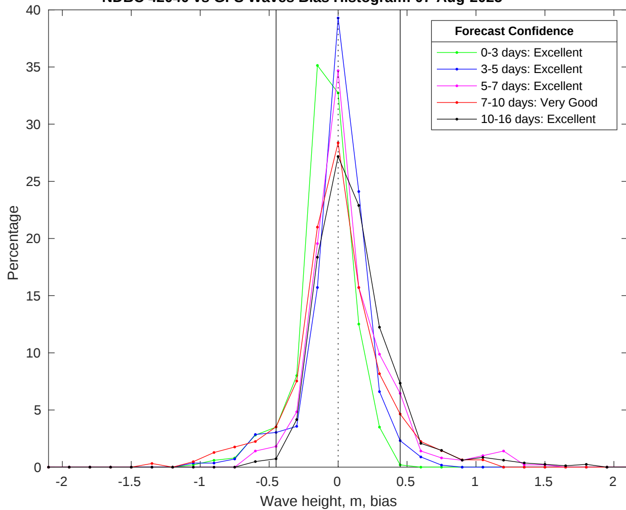
NDBC 42040 vs GFS Waves Bias Histogram: 07-Aug-2025
