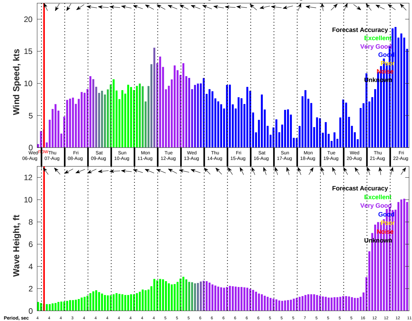
Wind & Wave Forecast for NDBC 42040 from 06-Aug-2025 19:00:00 to 22-Aug-2025 19:00:00
