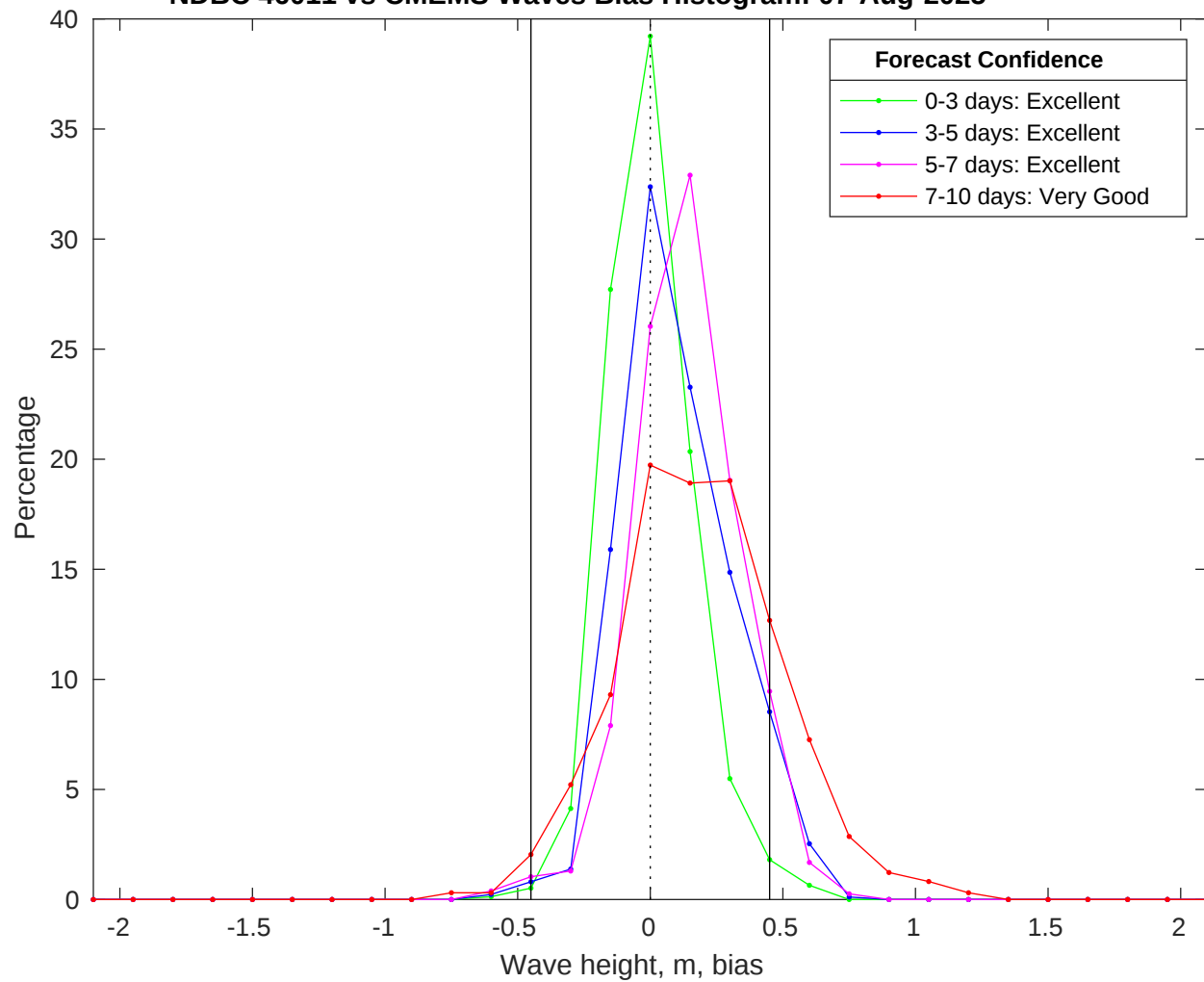
NDBC 46011 vs CMEMS Waves Bias Histogram: 07-Aug-2025
