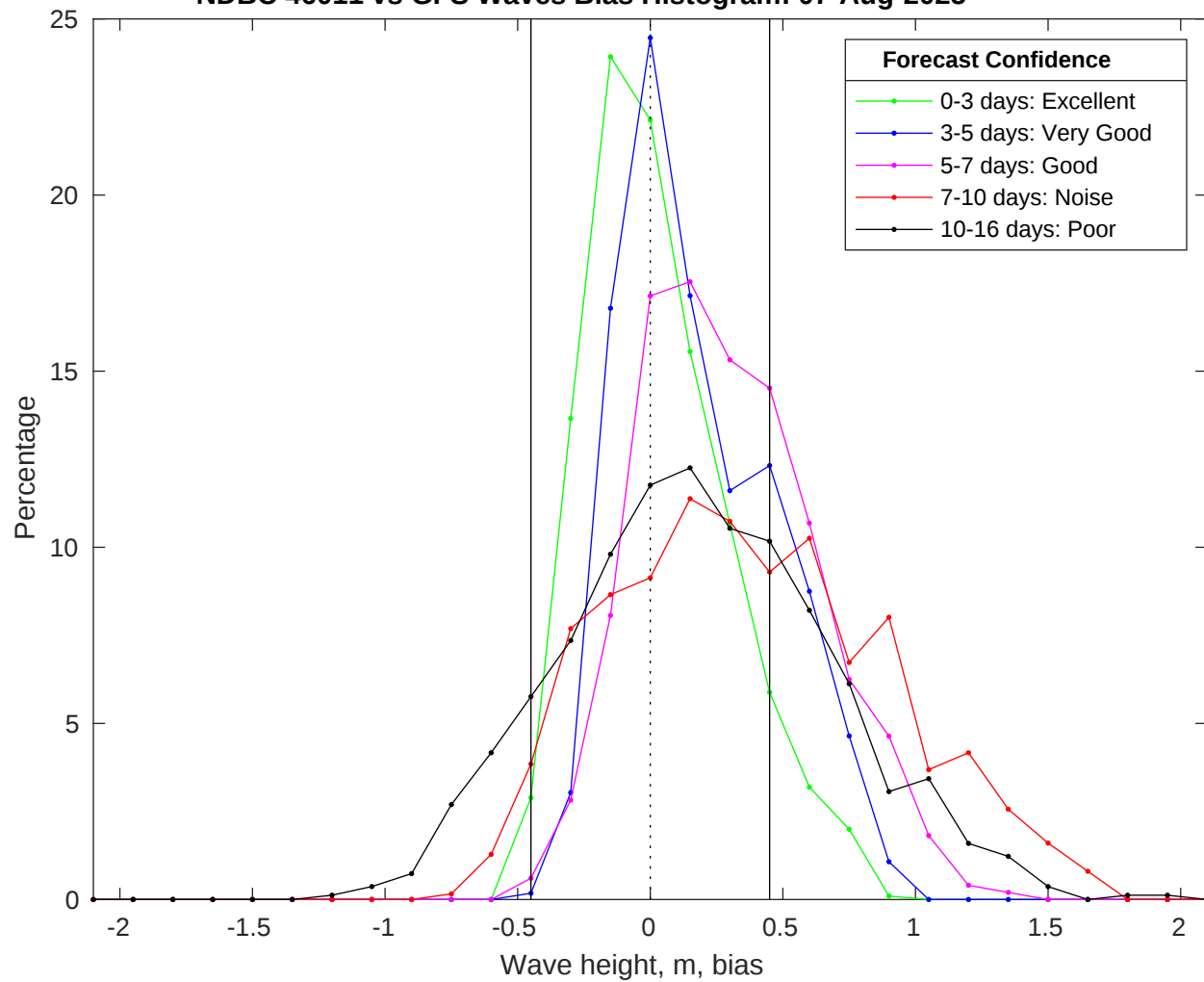
NDBC 46011 vs GFS Waves Bias Histogram: 07-Aug-2025
