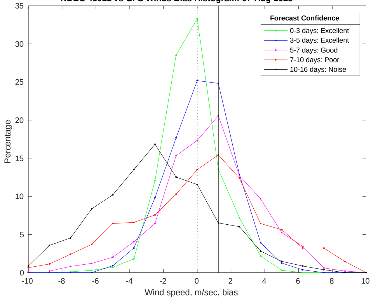
NDBC 46011 vs GFS Winds Bias Histogram: 07-Aug-2025
