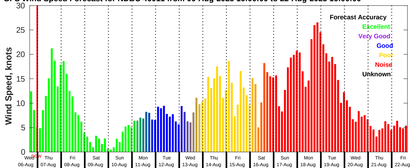
GFS Wind Speed Forecast for NDBC 46011 from 06-Aug-2025 16:00:00 to 22-Aug-2025 16:00:00
