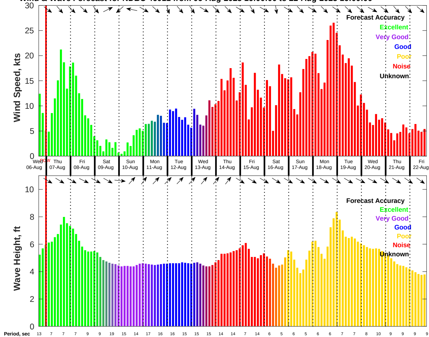
Wind & Wave Forecast for NDBC 46011 from 06-Aug-2025 16:00:00 to 22-Aug-2025 16:00:00
