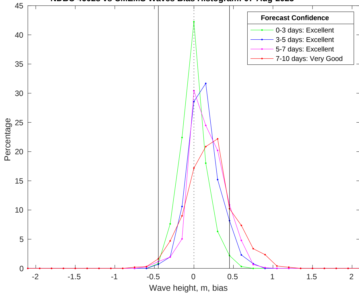
NDBC 46028 vs CMEMS Waves Bias Histogram: 07-Aug-2025
