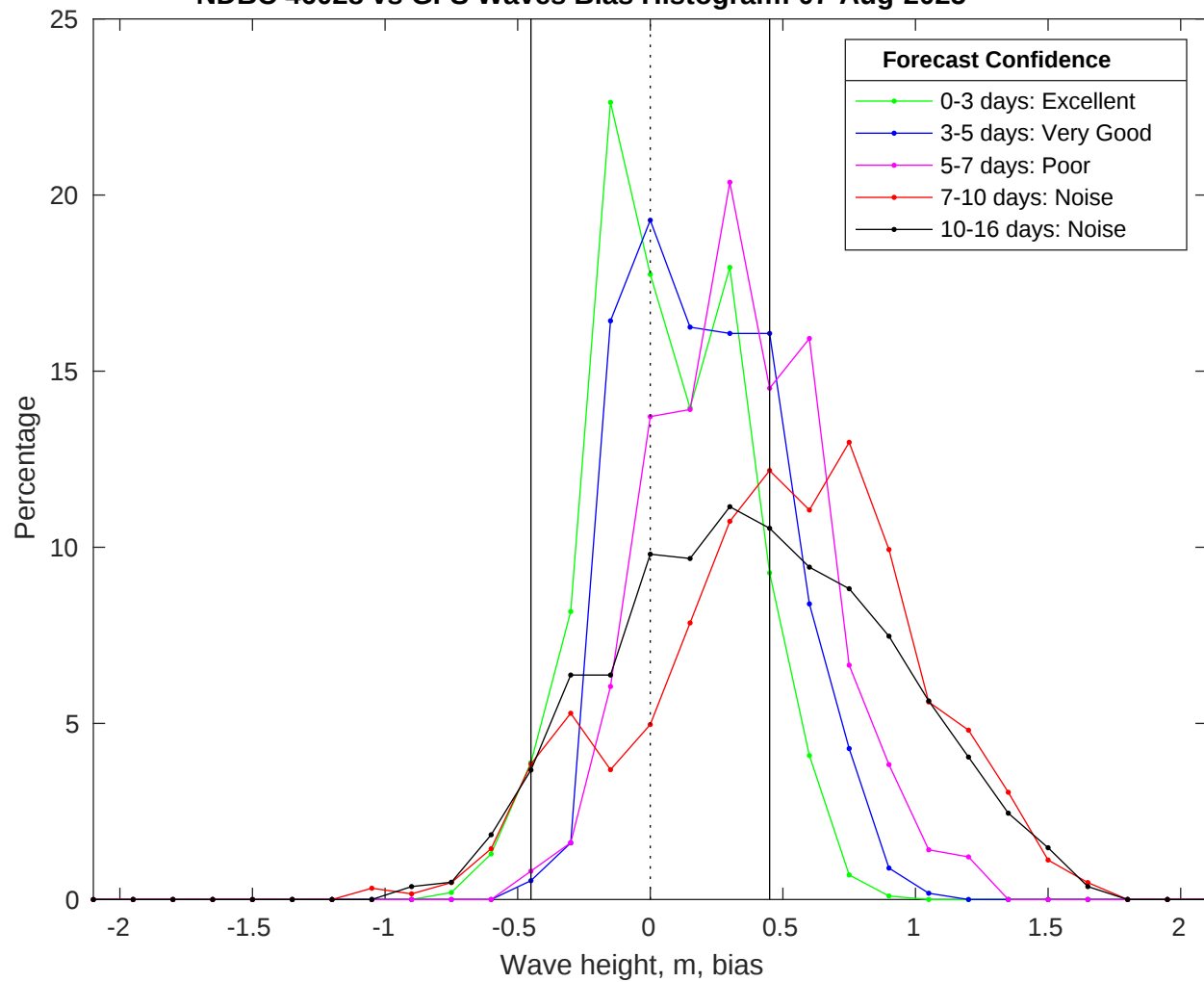
NDBC 46028 vs GFS Waves Bias Histogram: 07-Aug-2025
