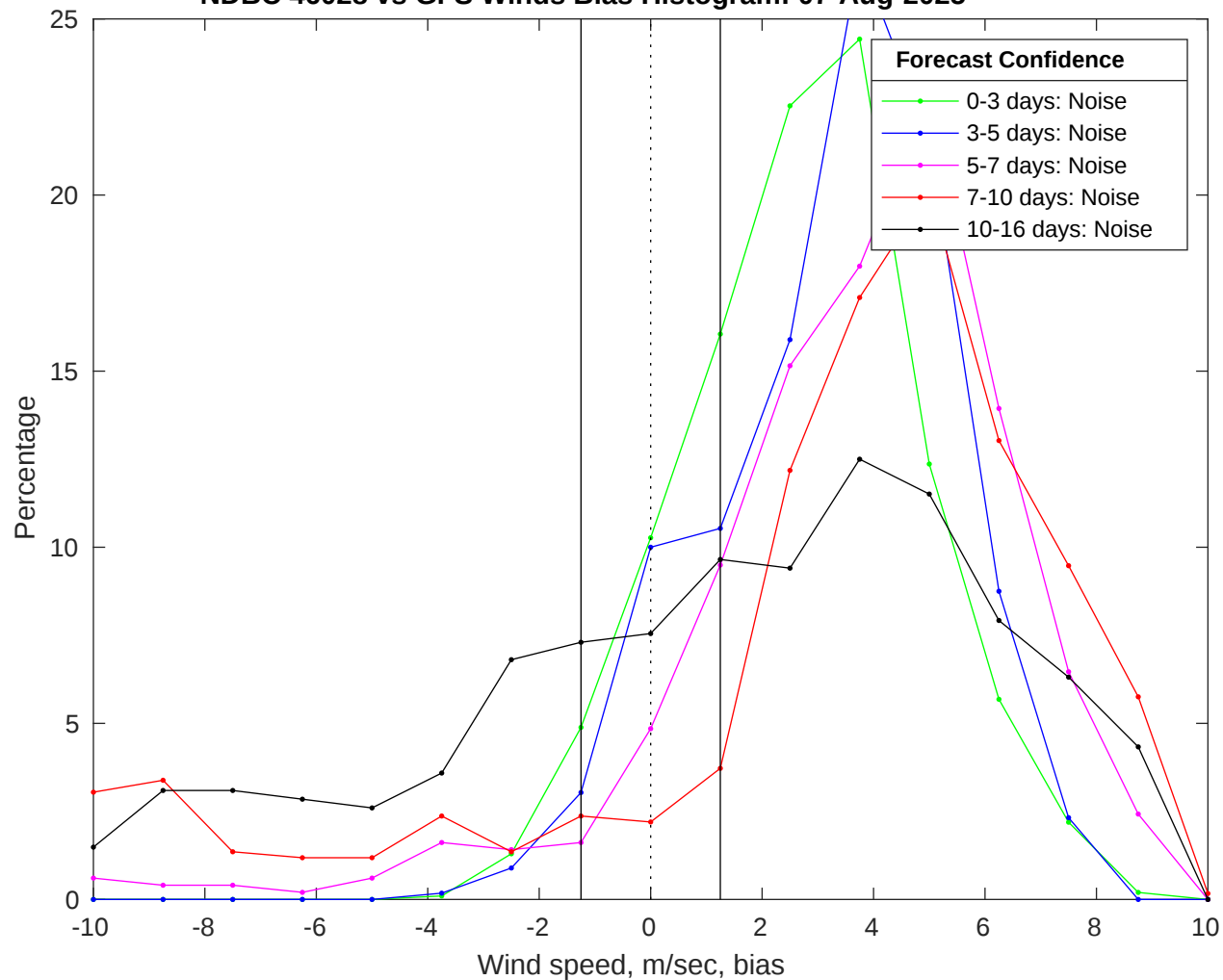
NDBC 46028 vs GFS Winds Bias Histogram: 07-Aug-2025
