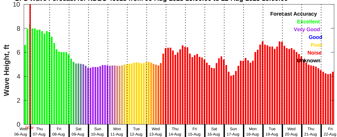
GFS Wave Forecast for NDBC 46028 from 06-Aug-2025 16:00:00 to 22-Aug-2025 16:00:00
